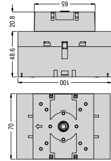
GA063 C...GA125 C
