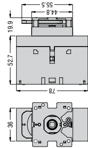
GA016 C...GA040 C
